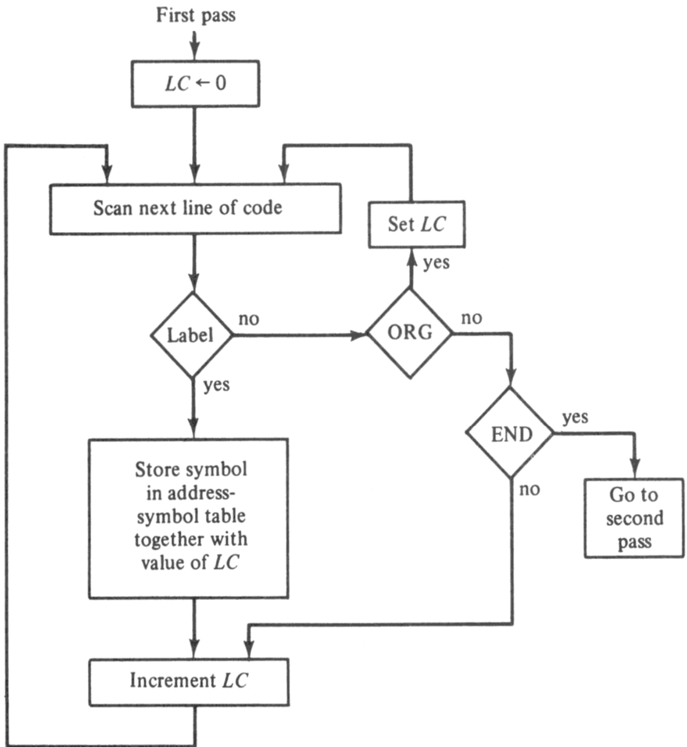
Figure 6-1 Flowchart for first pass of assembler.
