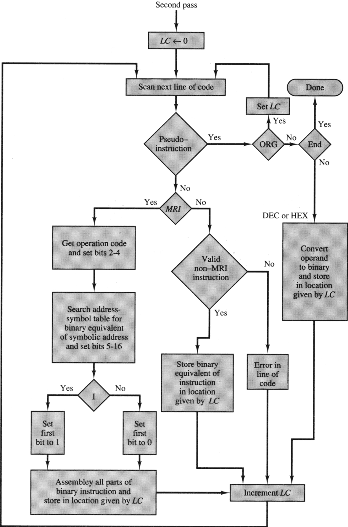
Figure 6-2 Flowchart for second pass of assembler.
